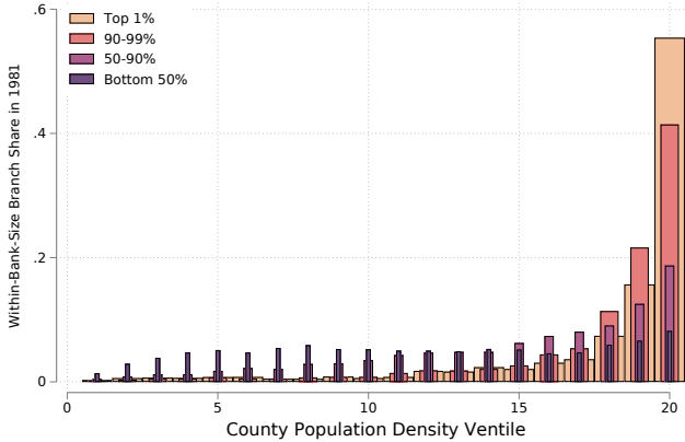
(a) Relative Sorting in 1981
