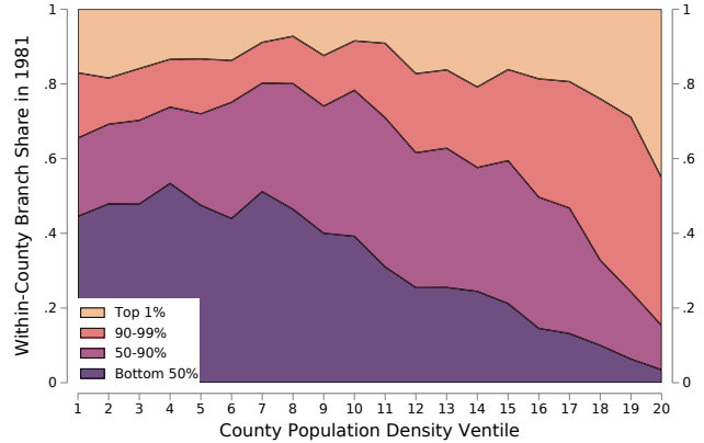
(b) Absolute Sorting in 1981
