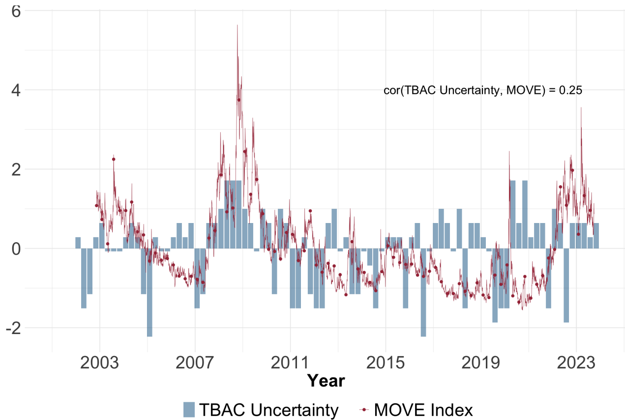
Figure A.7 Time Series of Uncertainty in TBAC Minutes Extracted from GPT-4o TBAC Uncertainty and MOVE time series are normalized to have mean 0 and variance 1.
