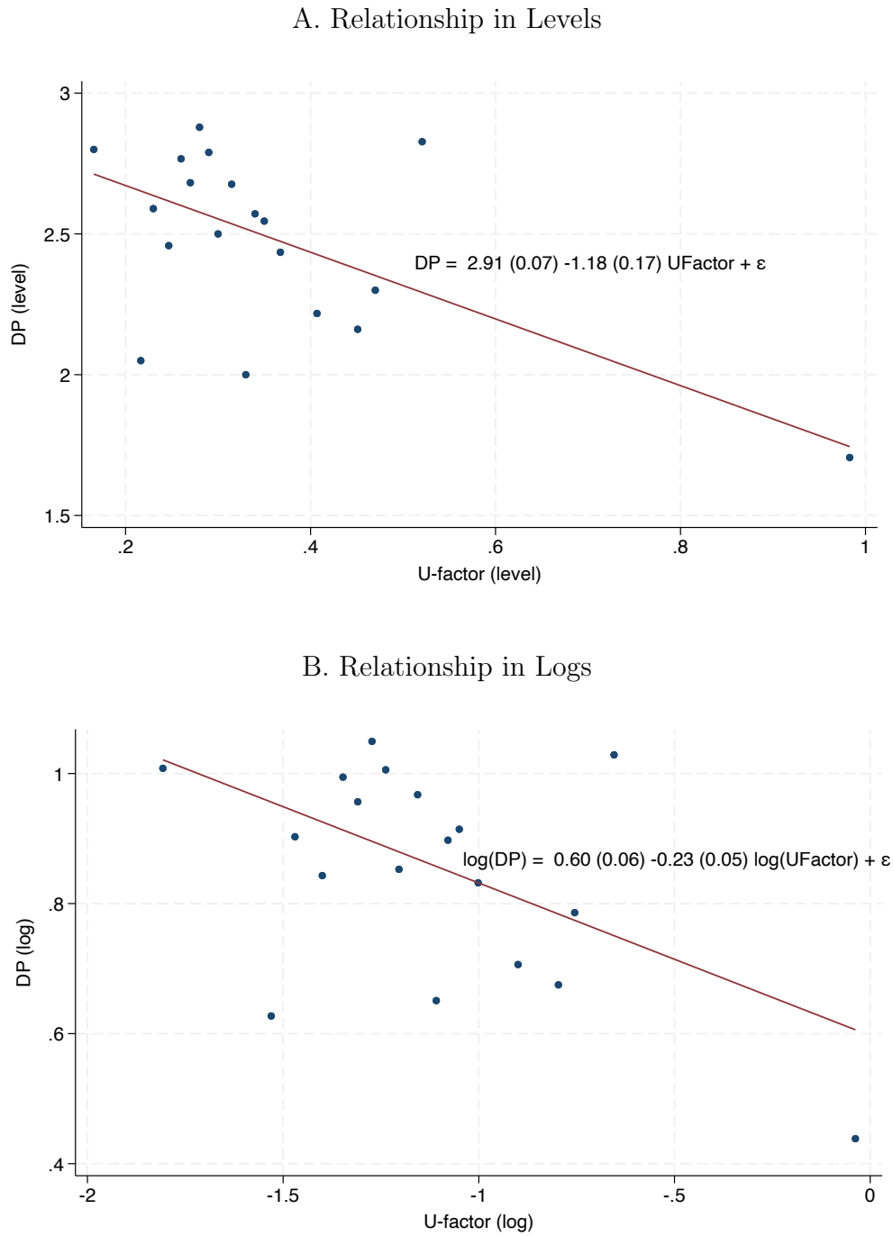
FIGURE 2. Relationship between Window Product DP Ratings and U-Factors
