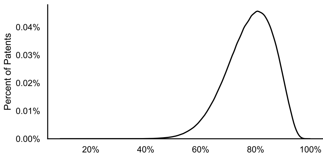
Panel B: KDE of Cosine Similarity Distribution
