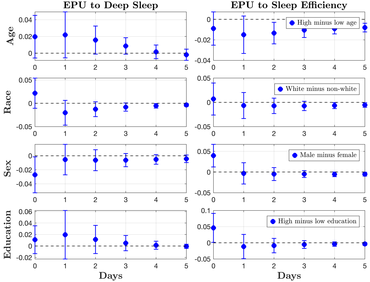
Figure 5: Impulse response functions: Heterogeneity by age, race, education, and sex The figure reports impulse response functions (IRFs) that display how a structural shock to economic uncertainty, measured using the natural logarithm of the daily Economic Policy Uncertainty (EPU) index of Baker et al. (2016), propagates to the difference in one of the two measures of sleep quality between two populations of interest. In the left panel, we measure sleep quality using the proportion of deep sleep, obtained via equation (1), while the right panel focuses on efficiency (right panel), obtained via equation (2). The first row looks at the difference in sleep quality between individuals in the top versus bottom quintile of age. The second row looks at the difference in sleep quality between white versus non-white individuals. The third row looks at the difference in sleep quality between individuals living in areas in the top versus bottom quintile of high school completion rates. The bottom row looks at the difference in sleep quality between male versus female individuals. A definition of each of these variables is provided in Section IA.A of the Internet Appendix. IRFs are obtained by estimating the vector autoregression presented by equation (6) and employing the recursive (Cholesky-based) identification of structural shocks. The solid blue line in each panel represents the average effect, and the 90% confidence interval represented by the blue-shaded region is obtained using a residual bootstrap with one thousand draws from the estimated residuals. Finally, the data underlying this analysis is daily and runs from April 26, 2017 through May 26, 2023.
