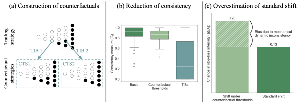
FIGURE 13.—Analysis of mechanical dynamic inconsistency
