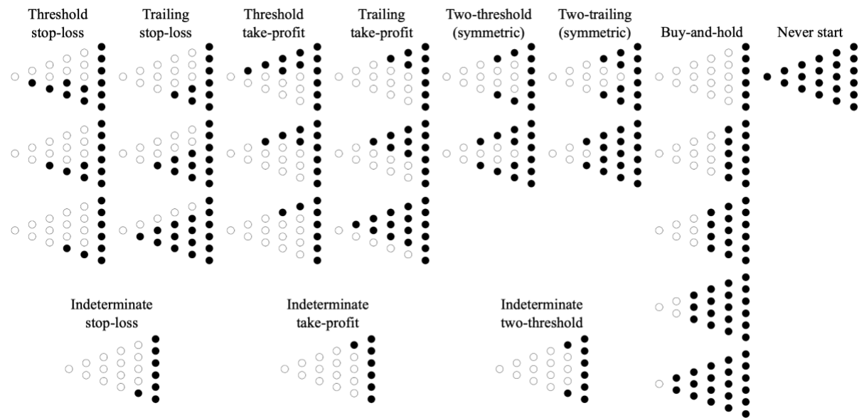
FIGURE SA.3.5.—All Basic risk-taking strategies for each class label
